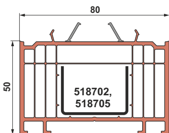
875050 80 Expander 80/50
