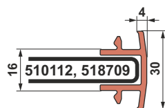
805002 58 71 80 Weather bar connector
