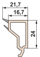
874644 Glass bead (glass unit 42 mm)
