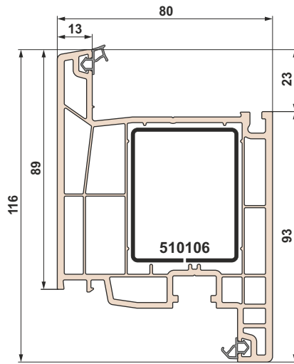
872040* Door sash of inside opening
