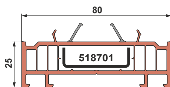
875025 80 Expander 80/25
