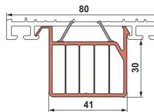
876030 80 Rafter plate (Mauerlat) 80/30
