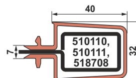
805003 58 71 80 Pilaster connector
