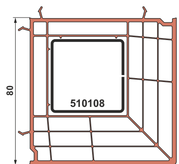
875120* 80 Corner connector 90°
