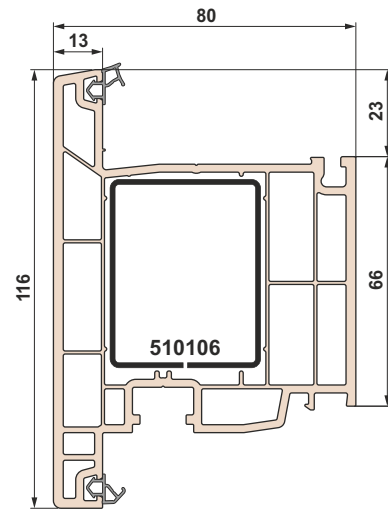
872020* Door sash of outside opening
