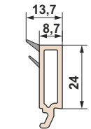
874652 Glass bead (glass unit 52 mm)
